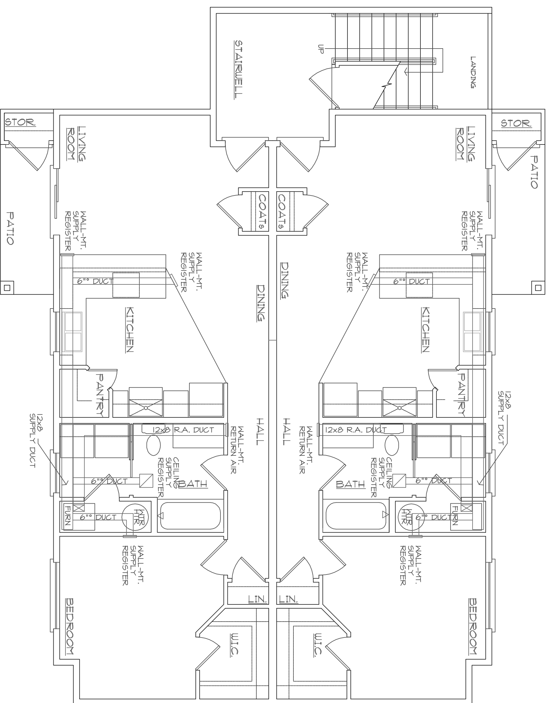
HVAC DUCT PLAN SINGLE BEDROOM SCALE: 1/4" = 1'-0" TYPICAL, ALL THREE FLOORS
